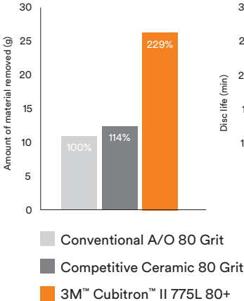
Cuts Faster! 6 minute material removal test
